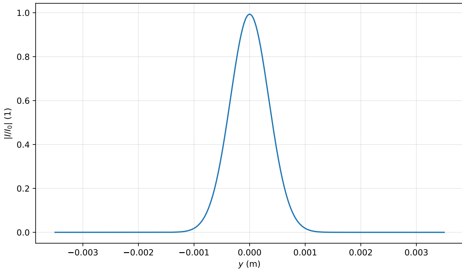
Intensity profile I(x=0, y, z=0.318)/I_0 , \text{Pin}=0.2\text{Pcr} , artificial time
